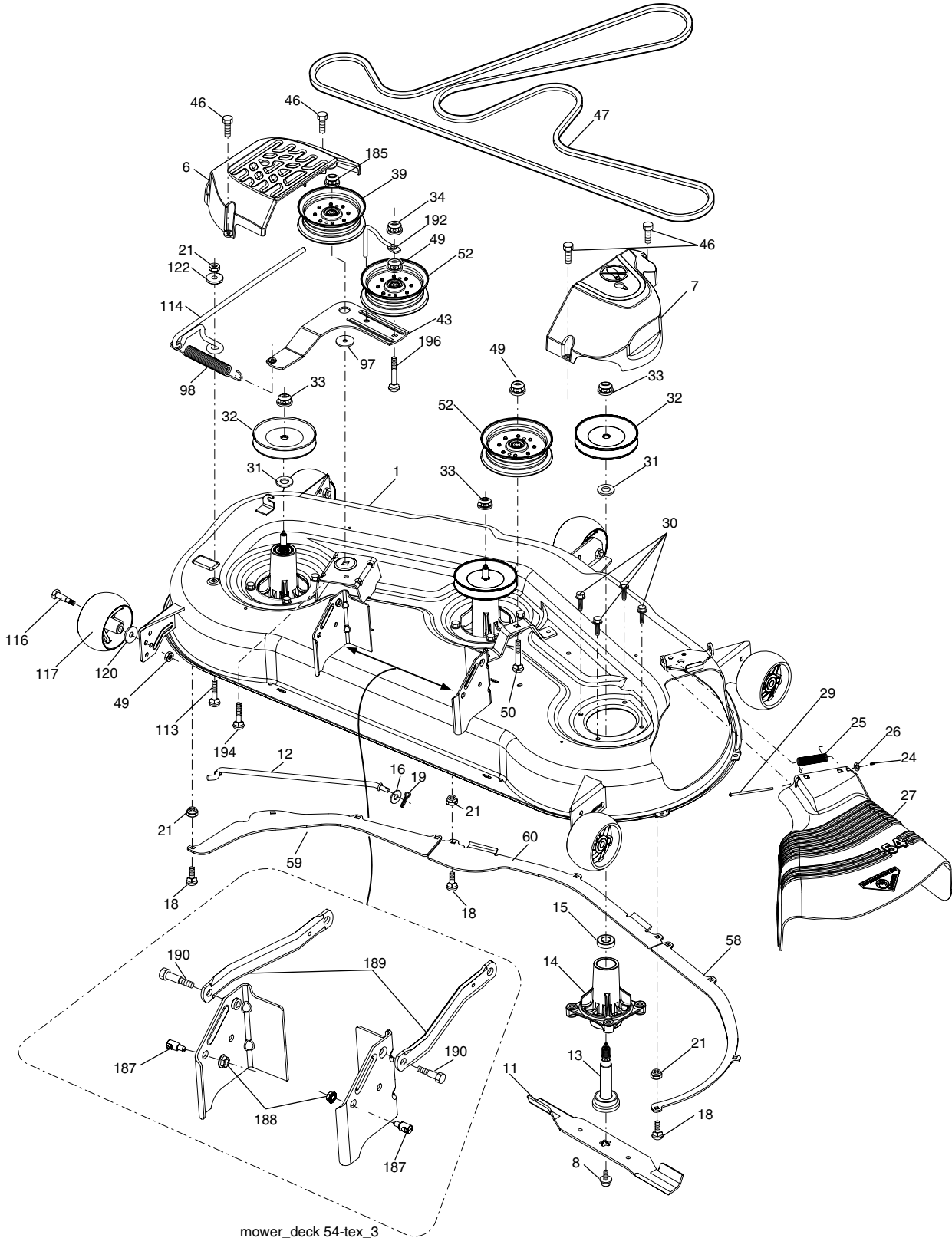
mower_deck 54-tex_3
