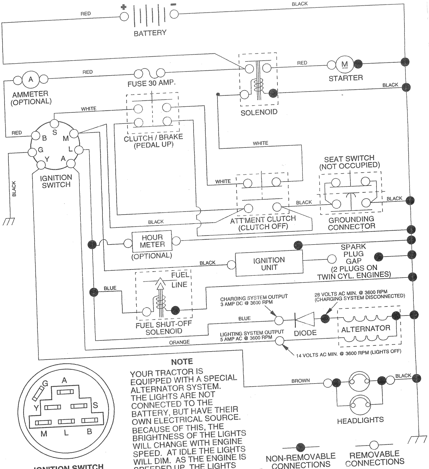
IGNITION SWITCH
